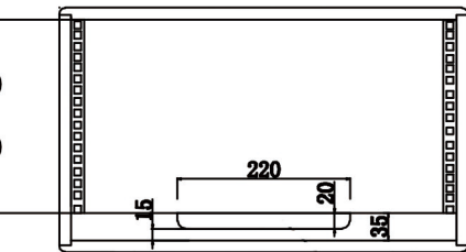
Back View
