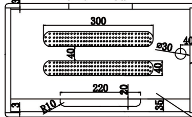
Back View
